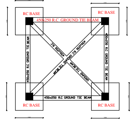
Foundation Plan
