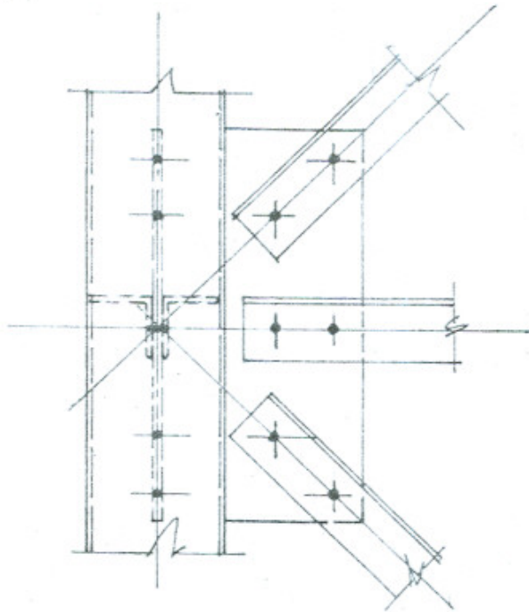
HORIZONTAL BRACINGS FIXING DETAIL. DETAIL Q'.
