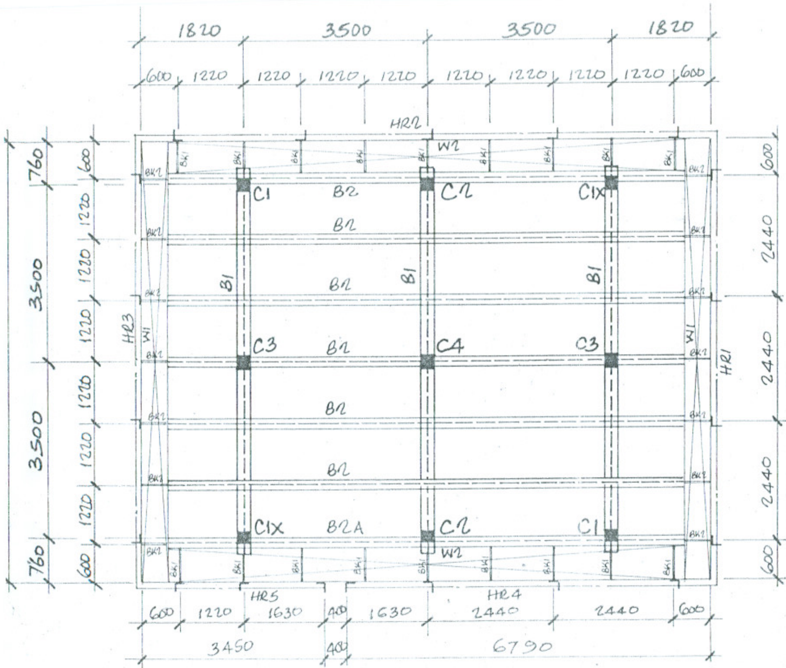
GENERAL ARRANGEMENT OF STEELWORK.
